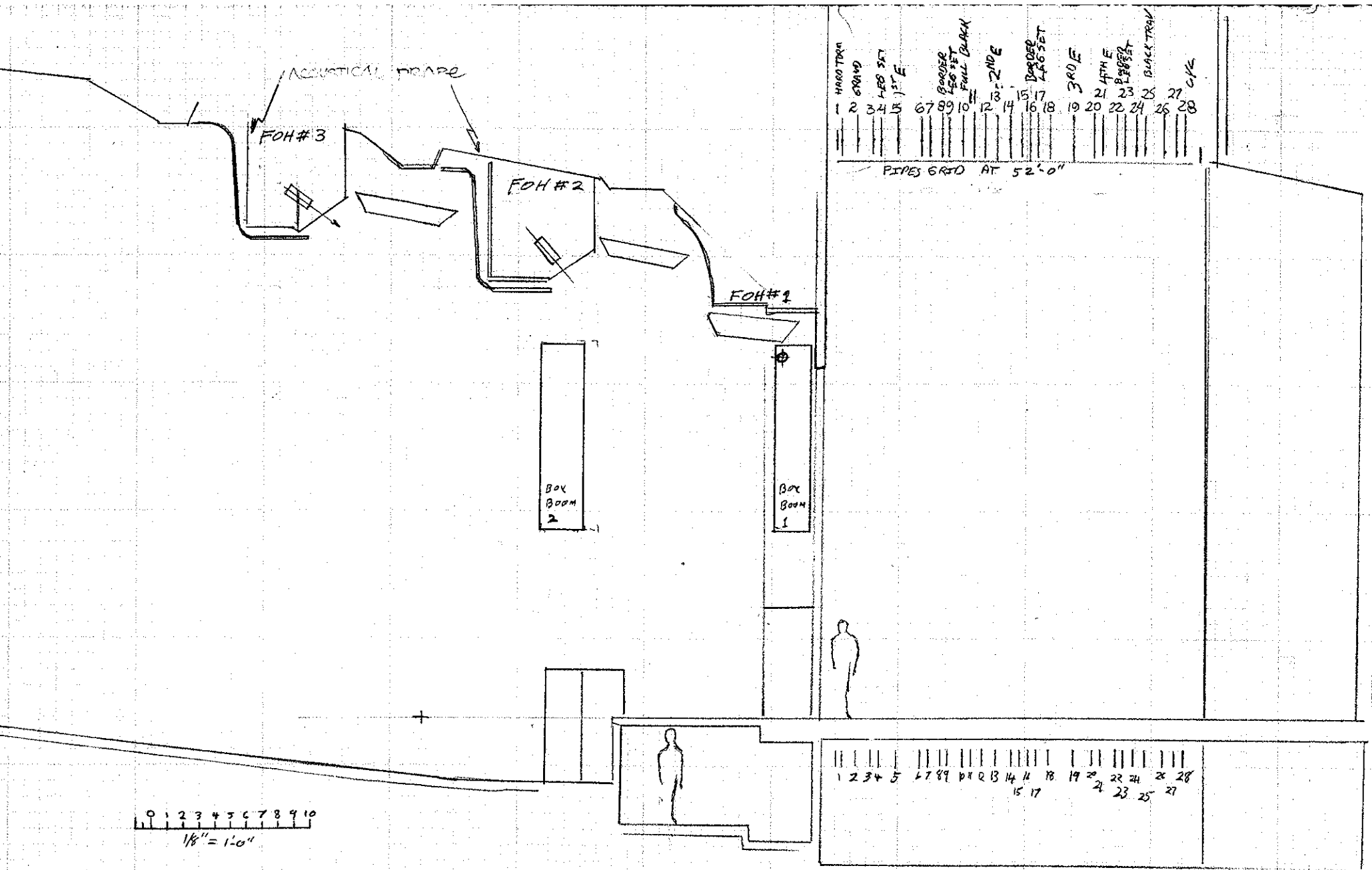
- HERING AUDITORIUM - SECTION - 1/8" = 1'-0" TRA FAIRBANKS, ALASKA
